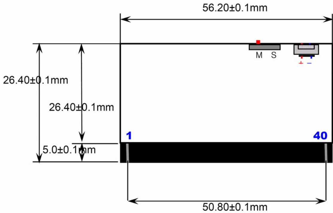
&lt; View from front side &gt;
