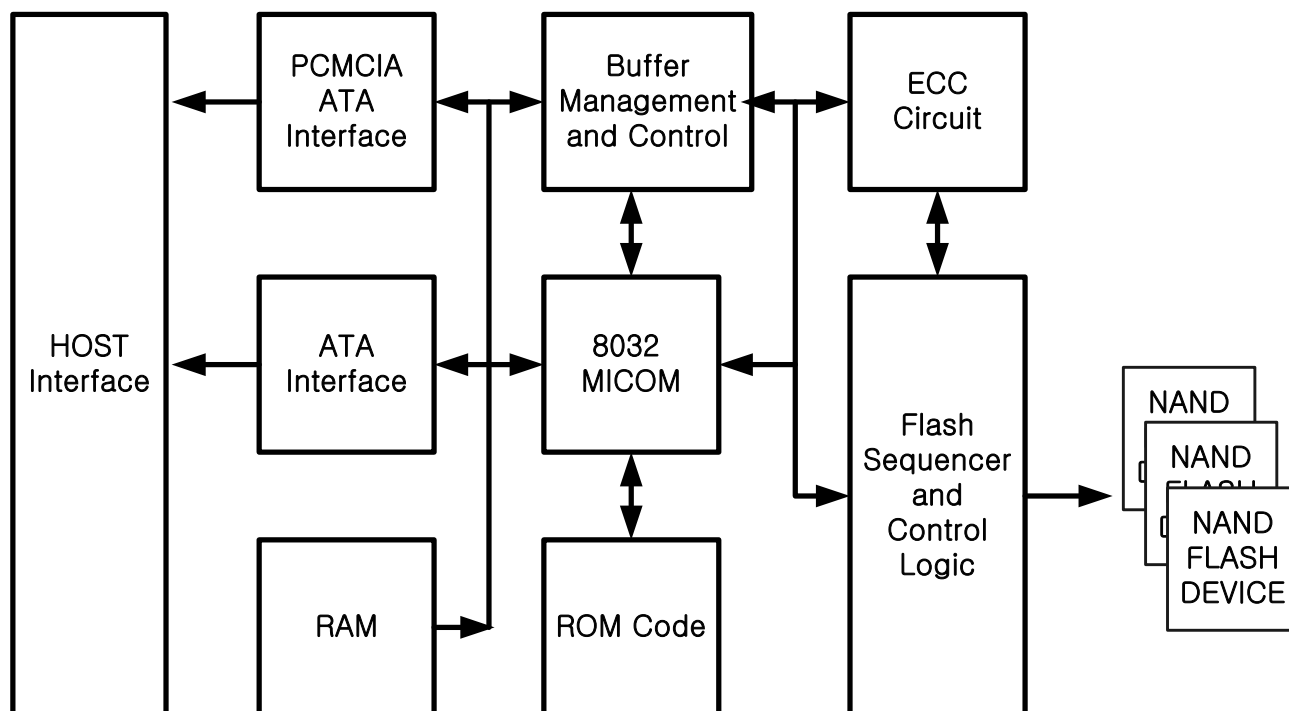
Figure 2.1 Block Diagram
