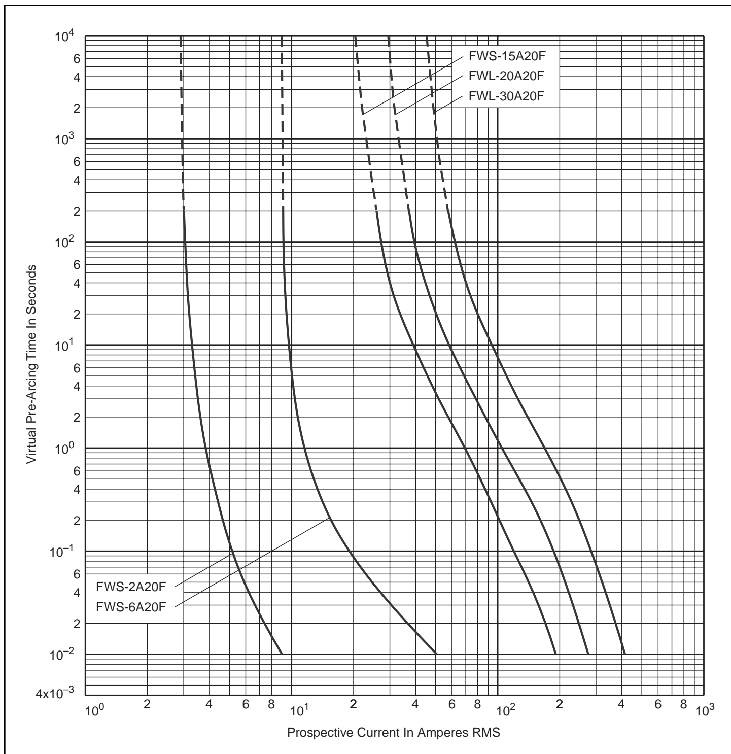
Minimum Melting Time-Current Characteristic Curves FWS 2A20F-15A20F FWL 20A2F-30A20F
