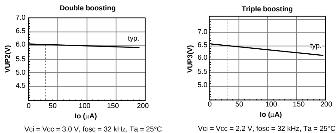
Figure 63 Booster (cont)
