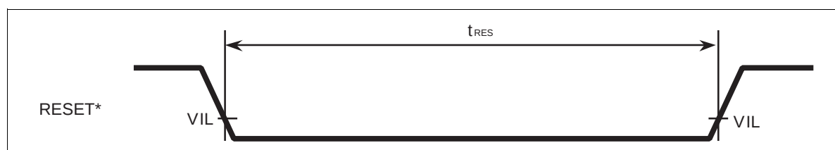
Figure 68 Reset Timing
