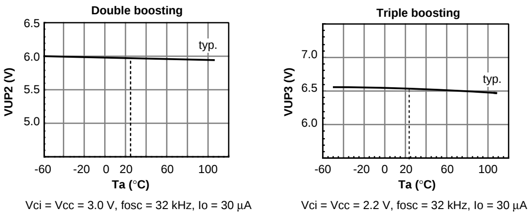
Figure 63 Booster (cont)
