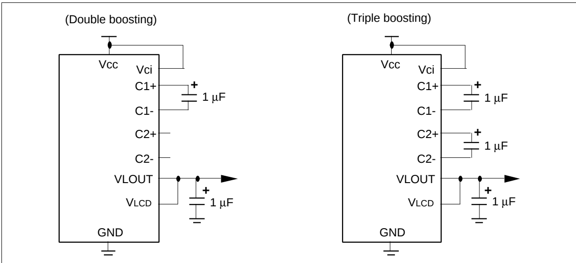
Figure 63 Booster
