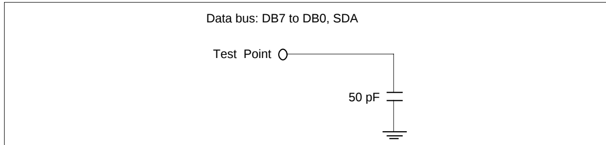
Figure 64 Load Circuit
