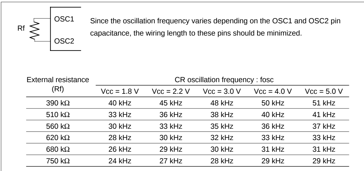
Figure 62 Internal Oscillation
