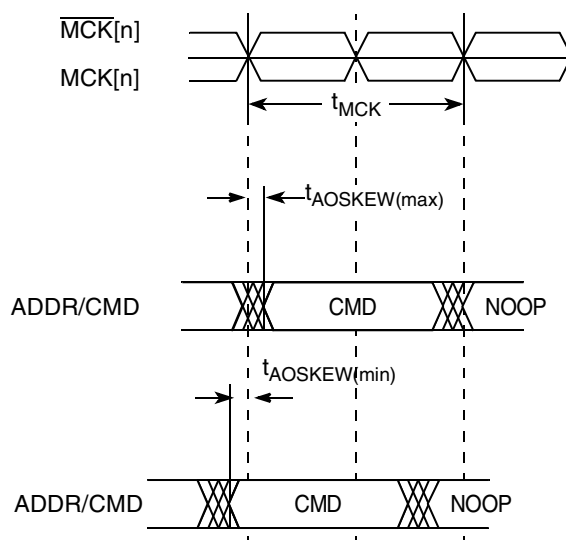
Figure 7. Timing Diagram for t_{\text{AOSKEW}} Measurement
