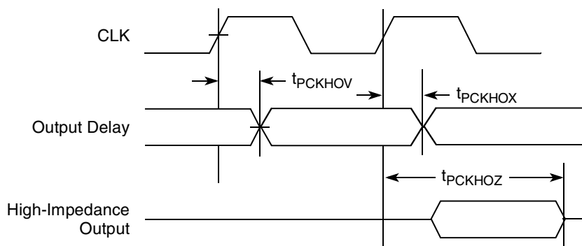
Figure 38. PCI Output AC Timing Measurement Condition
