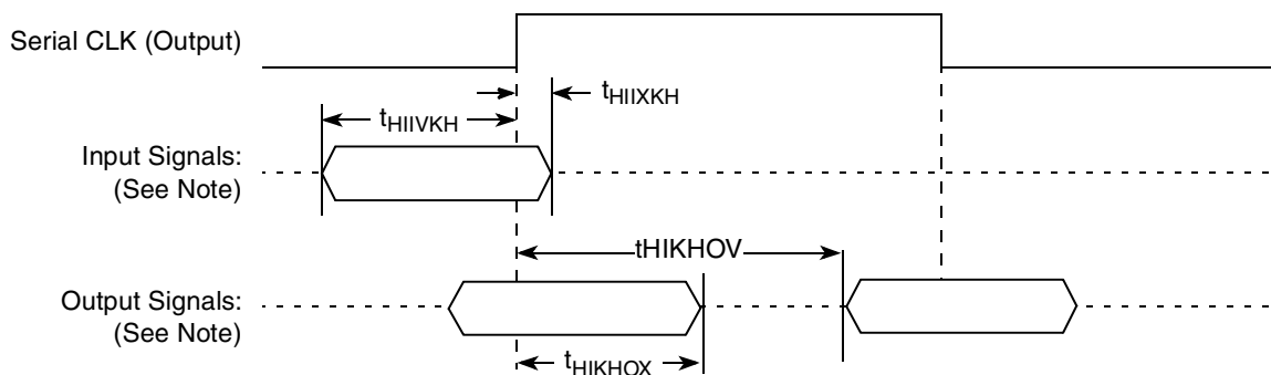
Figure 51. AC Timing (Internal Clock) Diagram
