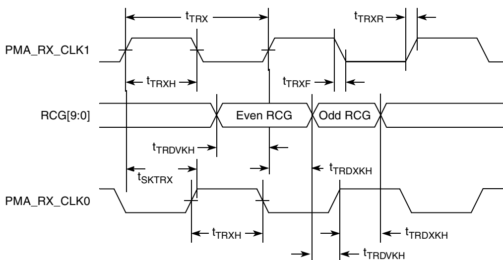
Figure 19. TBI Receive AC Timing Diagram
