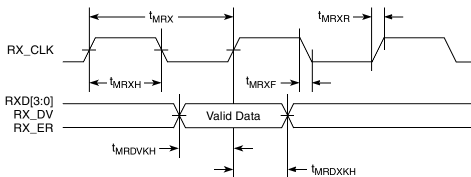
Figure 14. MII Receive AC Timing Diagram
