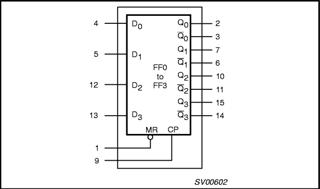
FUNCTIONAL DIAGRAM
