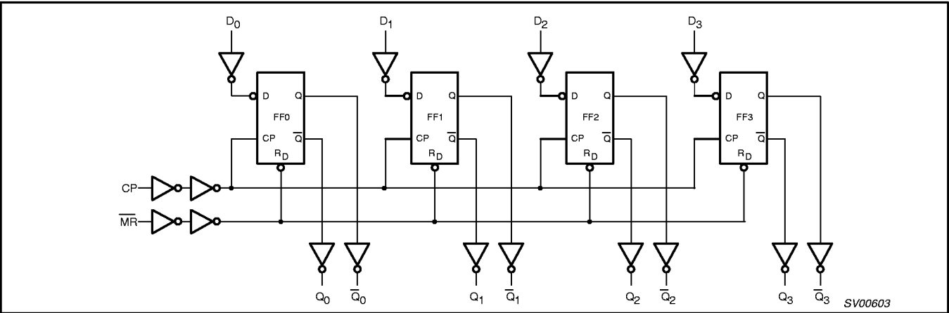
LOGIC DIAGRAM
