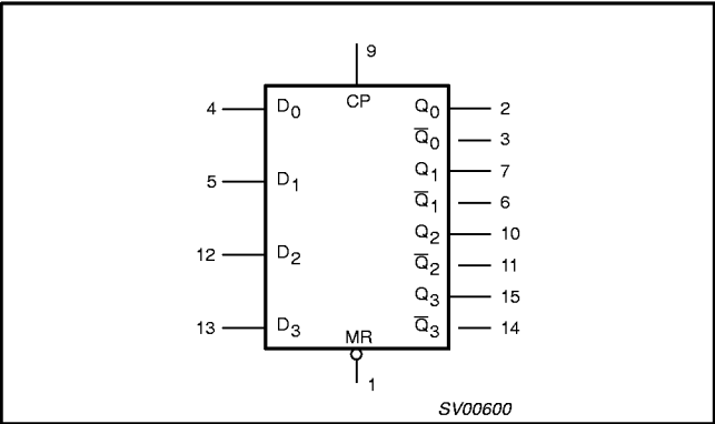
LOGIC SYMBOL
