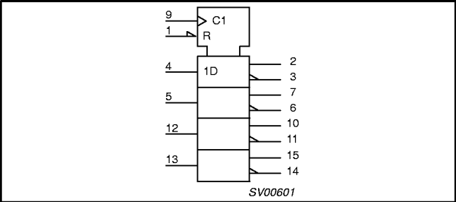
LOGIC SYMBOL (IEEE/IEC)
