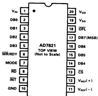
Q Package (DIP)
