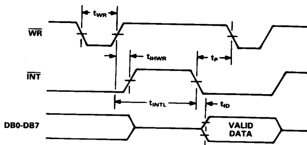
Figure 6. \overline{WR} - \overline{RD} Stand-Alone Operation, \overline{CS} = \overline{RD} = 0
