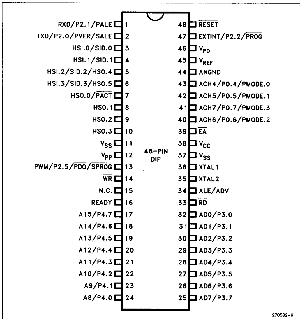
Figure 5. 48-Pin Package
