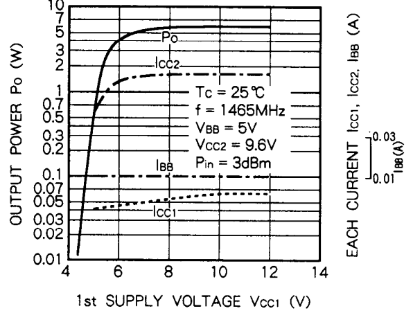
OUTPUT POWER, EACH CURRENT VS. 1st SUPPLY VOLTAGE CHARACTERISTICS
