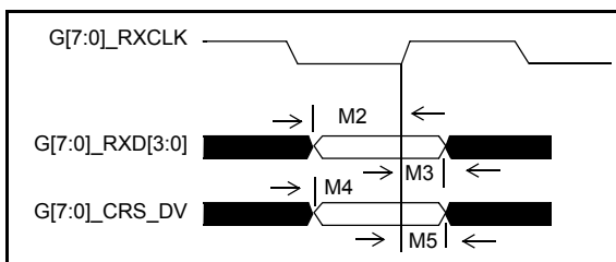
Figure 14 - AC Characteristics – Media Independent Interface
