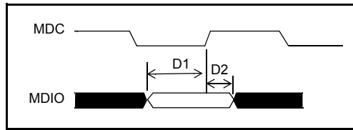
Figure 20 - MDIO Input Setup and Hold Timing
