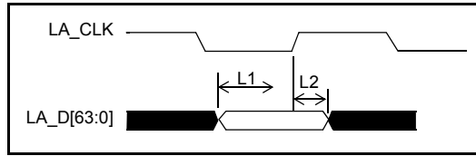
Figure 7 - Local Memory Interface – Input setup and hold timing
