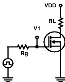
FIGURE 1. SWITCHING TIME TESTING
