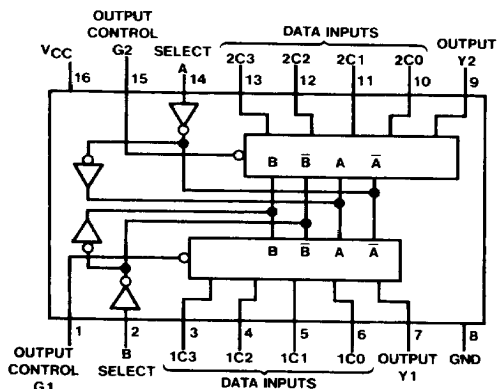
Dual-In-Line Package
