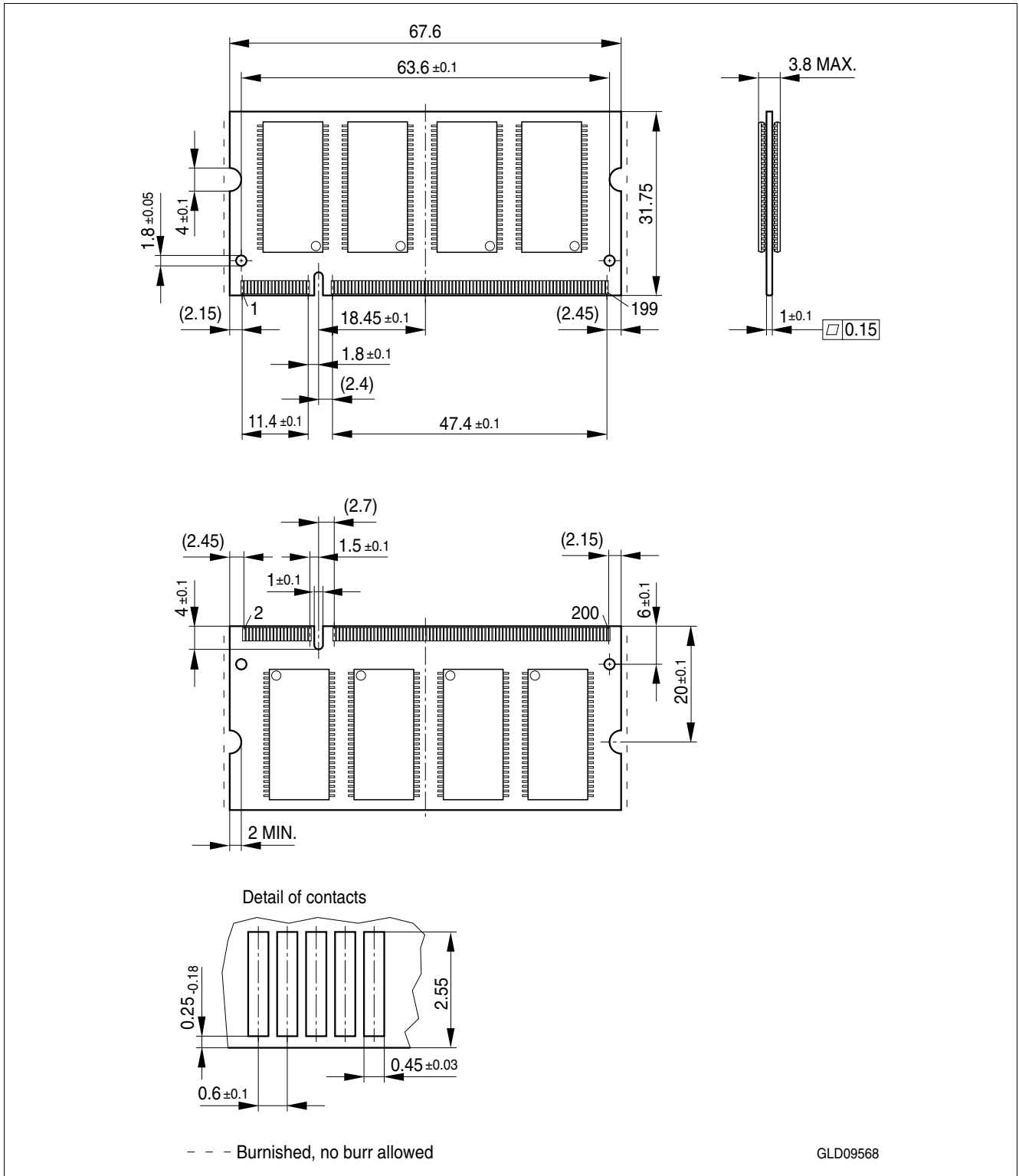
Figure 3 Package Outline SO-DIMM L-DIM-200-6
