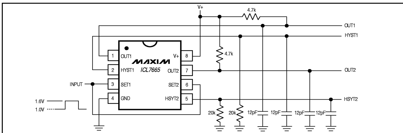
Figure 1. Test Circuit
