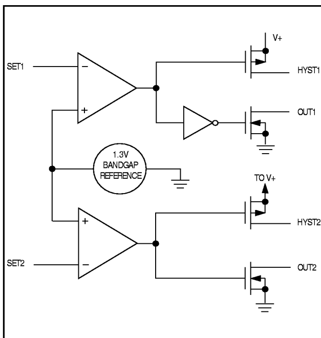
Figure 2. Block Diagram
