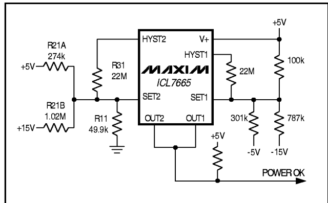
Figure 7. Multiple-Supply Fault Monitor
