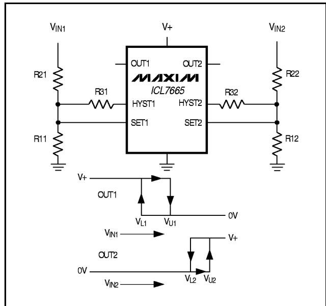
Figure 4. Threshold Detector with Hysteresis
