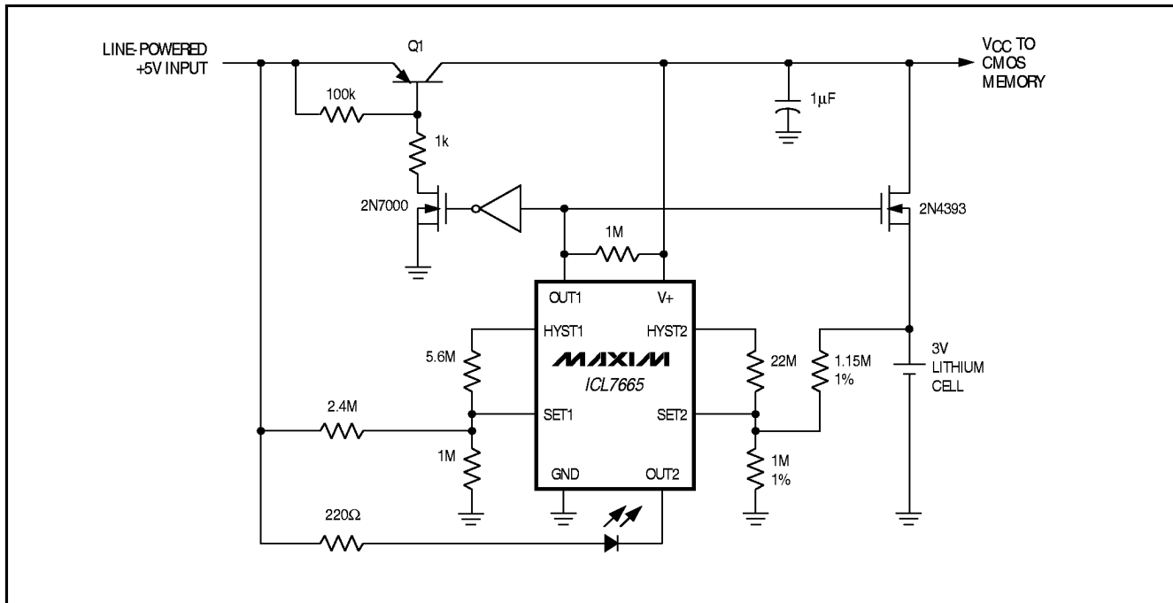
Figure 11. Battery Switchover Circuit
