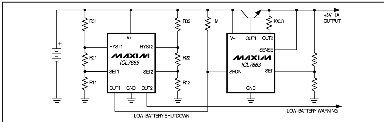
Figure 8. Low-Battery Warning and Low-Battery Disconnect
