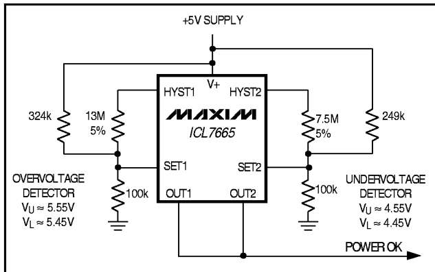
Figure 6. Fault Monitor for a Single Supply
