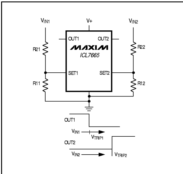
Figure 3. Simple Threshold Detector
