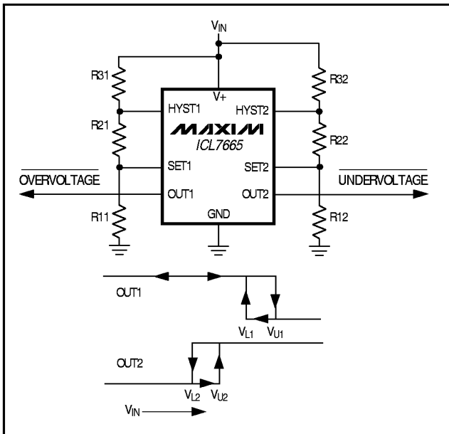
Figure 5. Threshold Detector, V_{IN} = V_+
