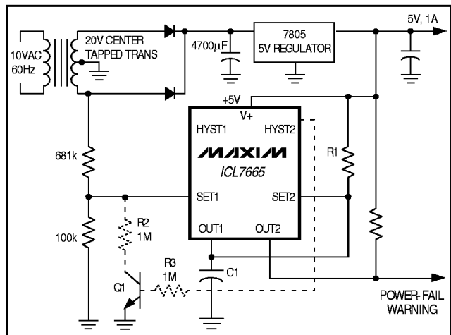
Figure 10. AC Power-Fail and Brownout Detector
