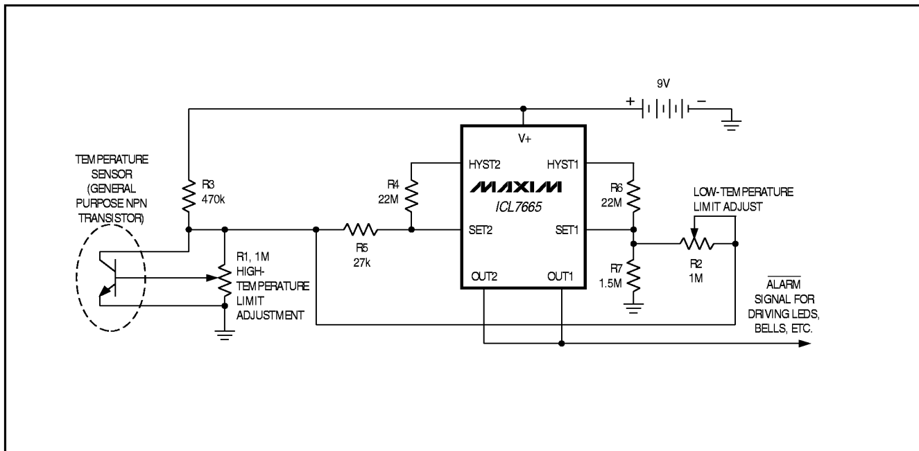
Figure 12. Simple High/Low Temperature Alarm
