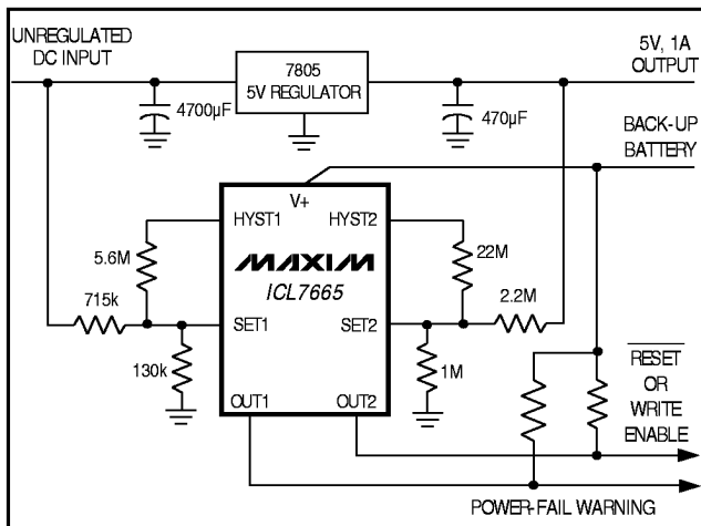
Figure 9. Power-Fail Warning and Power-Up/Power-Down Reset
