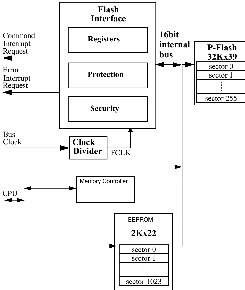
Figure 26-1. FTMRG128K1 Block Diagram
