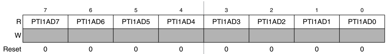
Figure 2-52. Port AD Input Register (PTI1AD)
