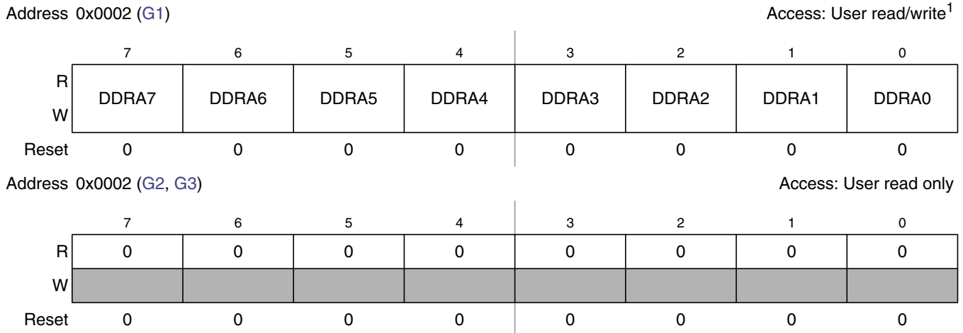
Figure 2-4. Port A Data Direction Register (DDRA)
