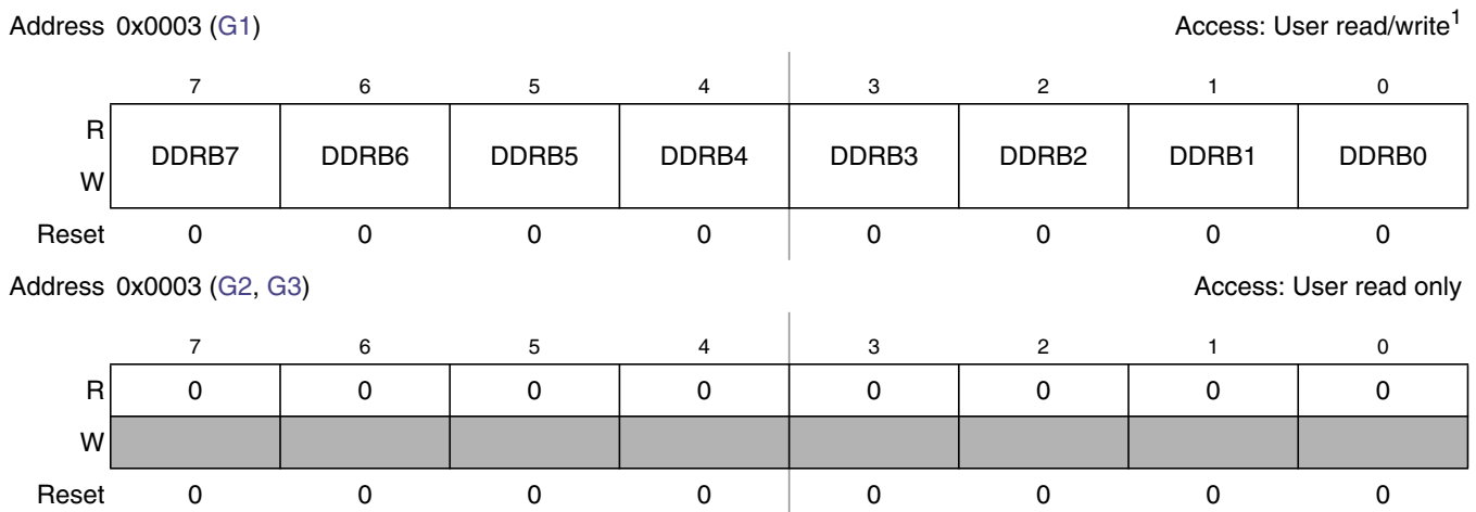
Figure 2-5. Port B Data Direction Register (DDRB)
