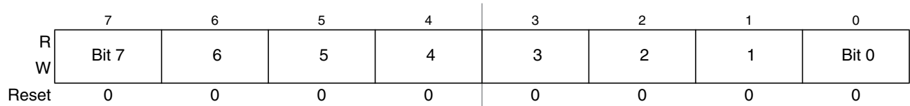
Figure 17-10. PWM Scale A Register (PWMSCLA)
