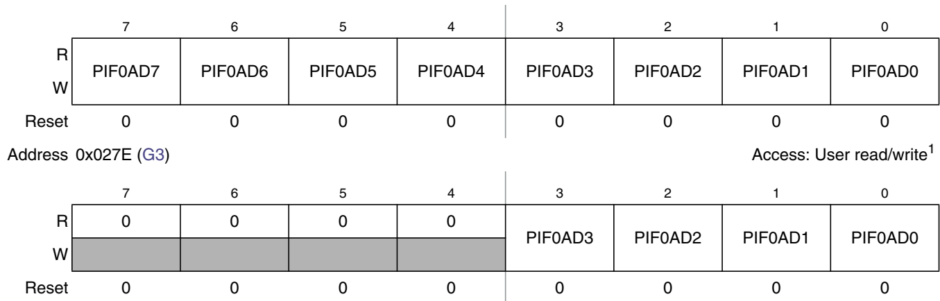
Figure 2-62. Port AD Interrupt Flag Register (PIF0AD)
