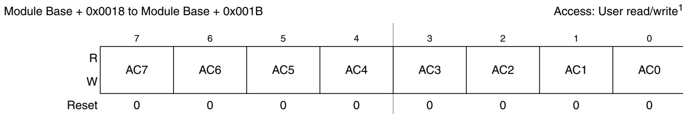
Figure 16-21. MSCAN Identifier Acceptance Registers (Second Bank) — CANIDAR4–CANIDAR7
