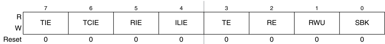
Figure 18-9. SCI Control Register 2 (SCICR2)
