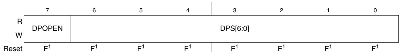
Figure 27-15. EEPROM Protection Register (EPROT)
