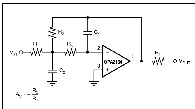
FIGURE 15. Dual Supply Filter Circuit.
