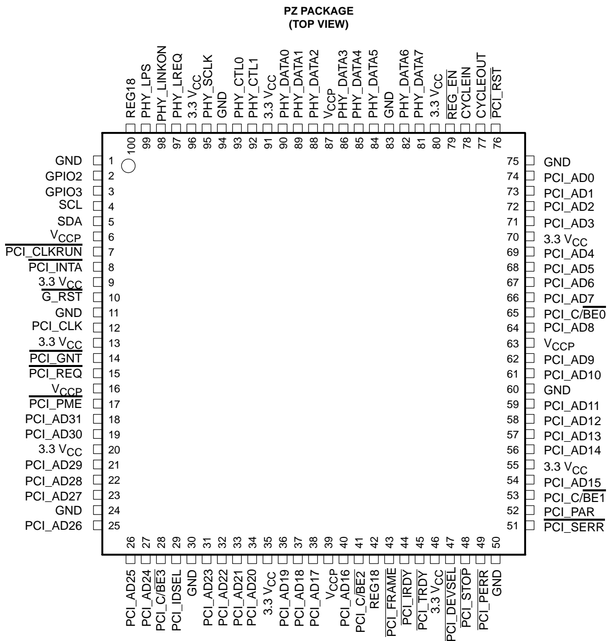
Figure 2–1. Terminal Assignments
