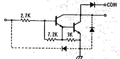
Dwg. No. A-9651
