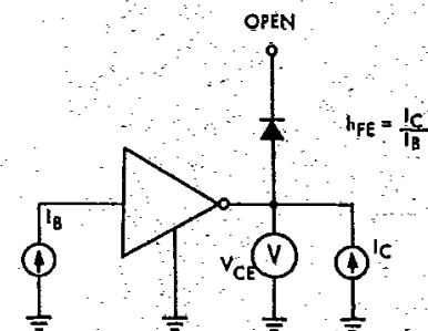
Dwg. No. A-9731
