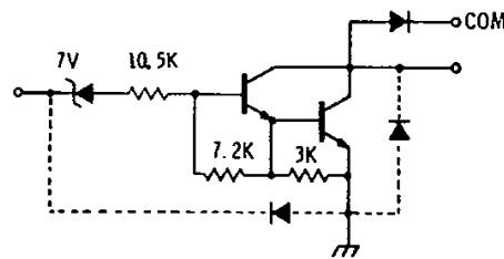
ULS20X2° (Each Driver)
