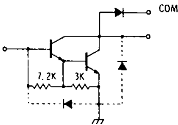
ULS20X1° (Each Driver)
