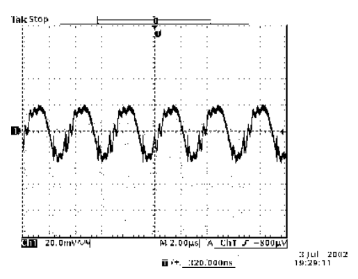
Ripple and noise at full load and 5Vdc input, 1.2Vdc output and Ta=25° C
