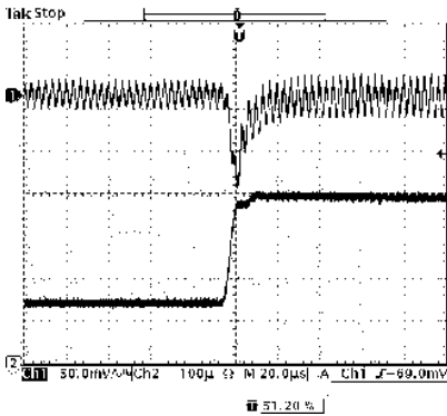
Vout=2.5V 50% to 100% load transients at 5V input and Ta=25° C
