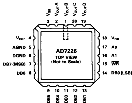
E Package (LCC)
