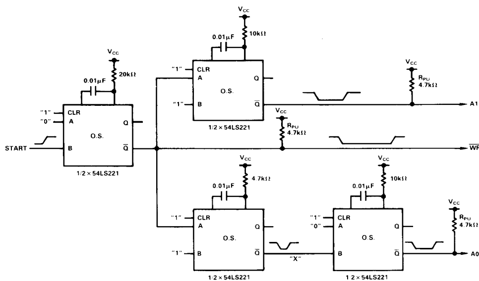
Figure 2. Initialization Circuit
