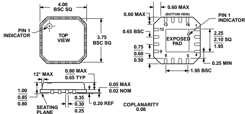
Figure 23. 16-Lead Lead Frame Chip Scale Package [LFCSP_VQ] 4 mm x 4 mm Body, Very Thin Quad (CP-16-4) Dimensions shown in millimeters
