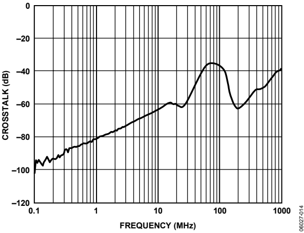
Figure 19. Crosstalk
