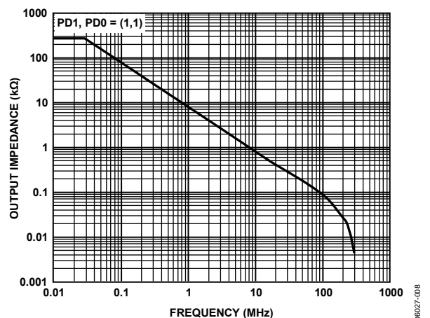
Figure 17. Output Impedance vs. Frequency (Disabled)
