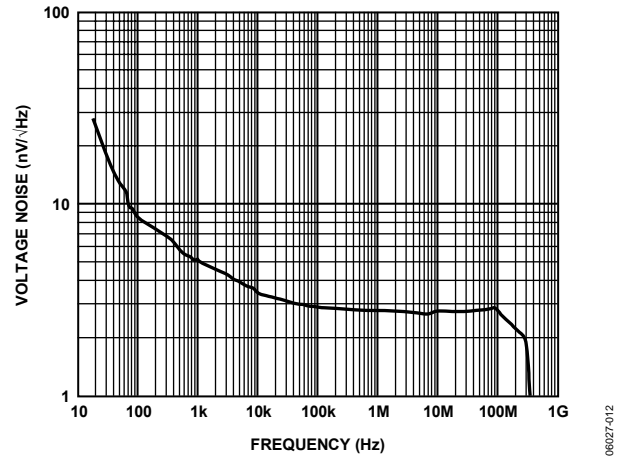
Figure 11. Voltage Noise vs. Frequency
