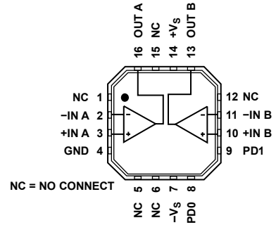
Figure 6. 16-Lead LFCSP Pin Configuration
