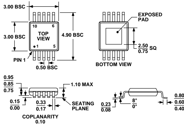
Figure 22. 10-Lead Mini Small Outline Package with Exposed Pad [MINI_SO_EP] (RH-10) Dimensions shown in millimeters
