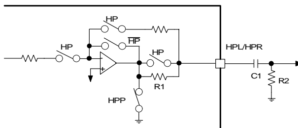
Figure 25. Headphone-Amps Power-Down-Mode
