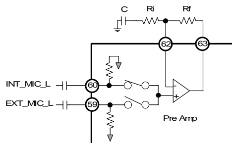
Figure 14. Pre-Amp
