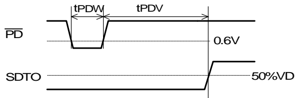
Figure 7. Reset Timing
