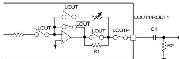
Figure 20. LINEOUT Power-Save-Mode
