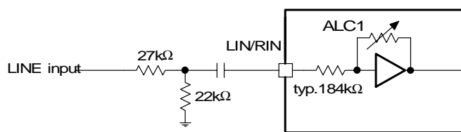
Figure 18. Example of LINEIN at VA=2.8V
