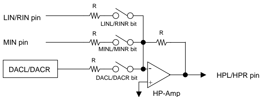
Figure 22. Summation circuit for headphone amp output
