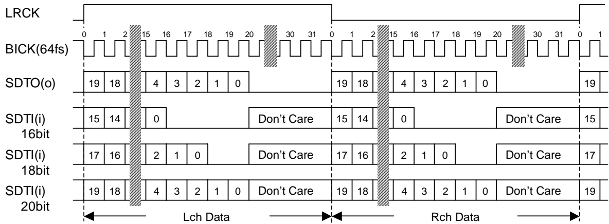
Figure 12. Mode 2 Timing
