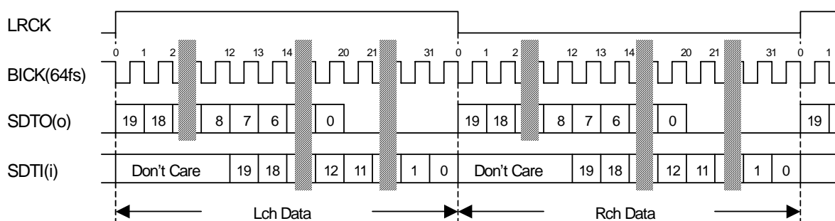
Figure 11. Mode 1 Timing
