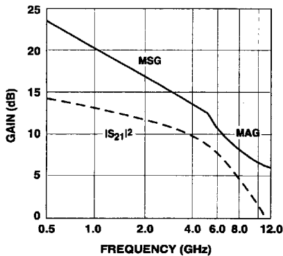
Figure 1. Insertion Power Gain, Maximum Available Gain and Maximum Stable Gain vs. Frequency. V_{DS} = 3\text{ V} , I_{DS} = 20\text{ mA} .
