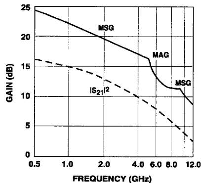
Figure 2. Insertion Power Gain, Maximum Available Gain and Maximum Stable Gain vs. Frequency. V_{DS} = 5\text{ V} , I_{DS} = 50\text{ mA} .
