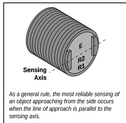
Figure 1. Sensing axis
