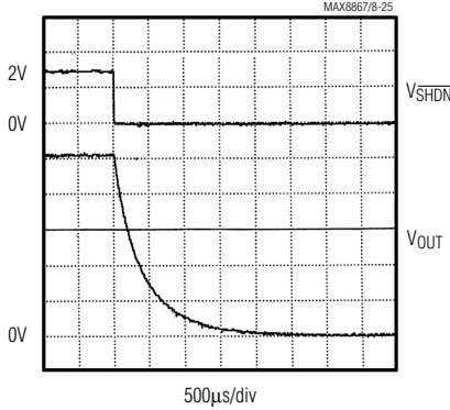
MAX8868 ENTERING SHUTDOWN
