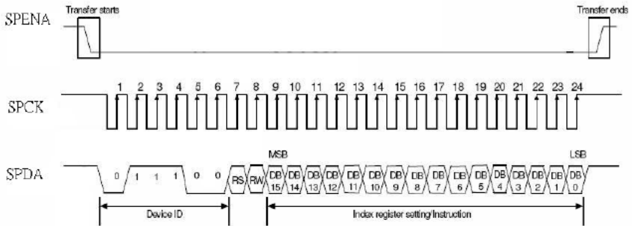
Figure10 SPI timing
