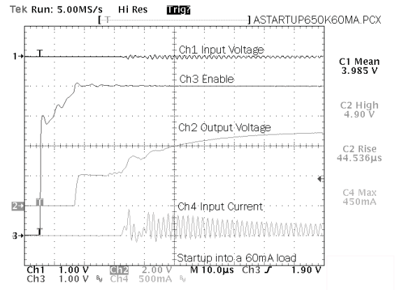
Start-Up Conditions for 5.0V Output
