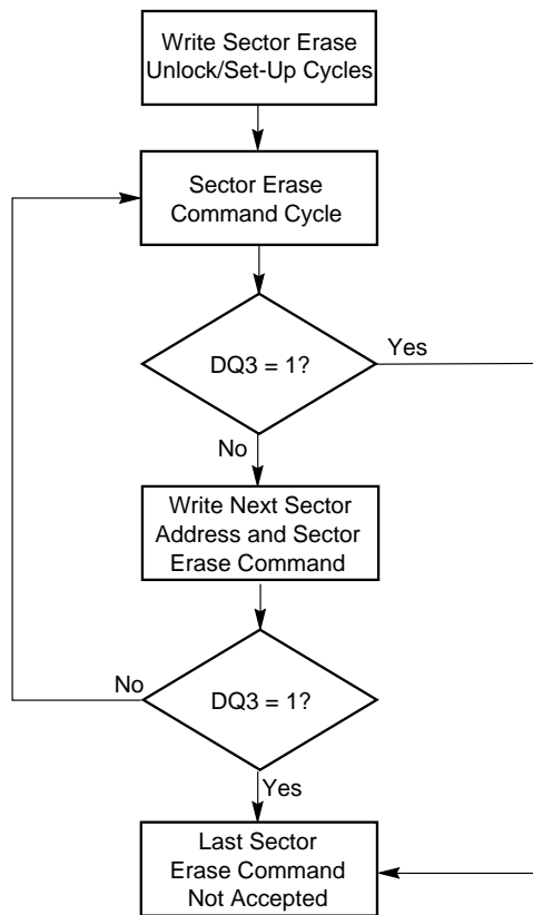
Figure 7. DQ3 Sector Erase Timer
