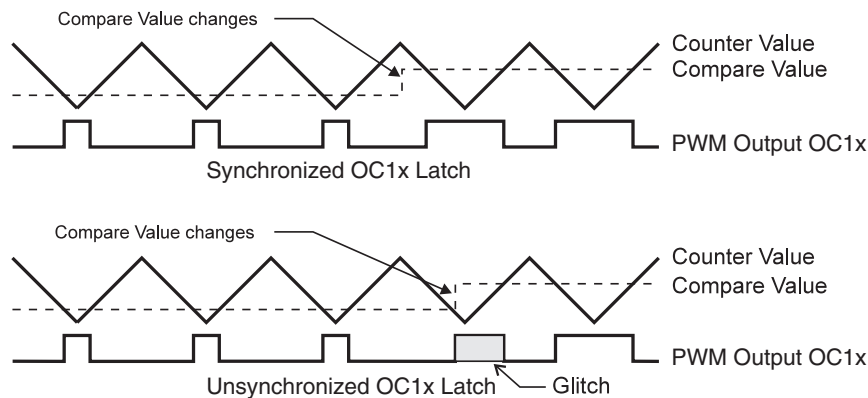
Figure 35. Effects of Unsynchronized OCR1 Latching.
