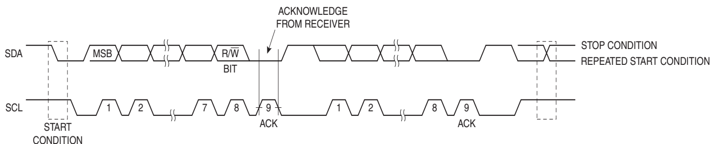
Figure 50. 2-wire Serial Bus Timing Diagram
