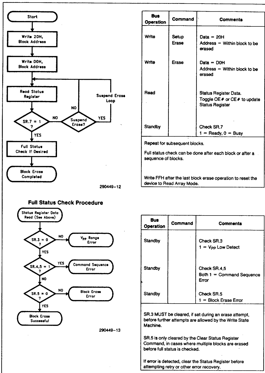
Figure 14. Automated Block Erase Flowchart
