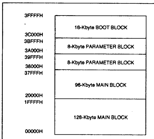
Figure 11. 28F002BX-TL Memory Map
