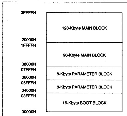
Figure 10. 28F002BX-BL Memory Map
