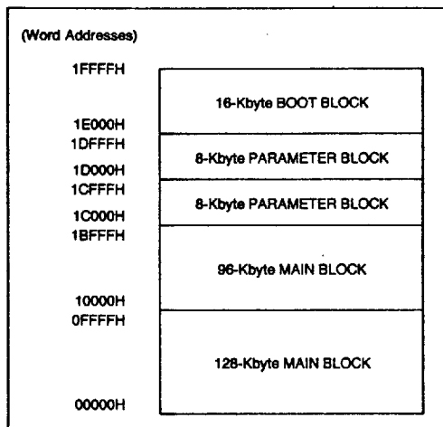
Figure 8. 28F200BX-TL Memory Map
