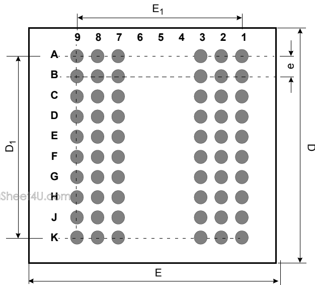
*2: Top View
