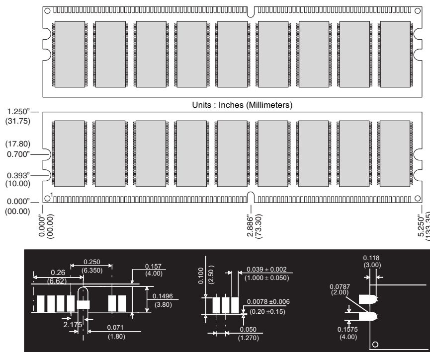
Figure 1: KVR400X72C3A/1G 184-Pin DDR SDRAM Module
