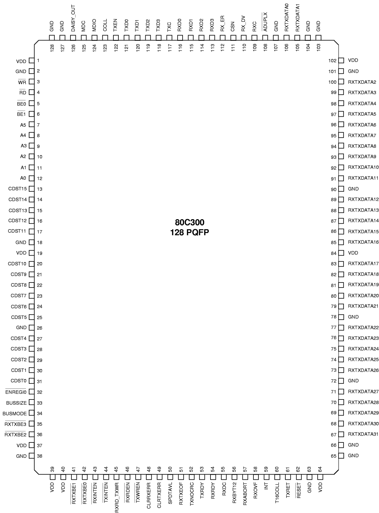
Figure 2. 80C300 Pin Configuration
