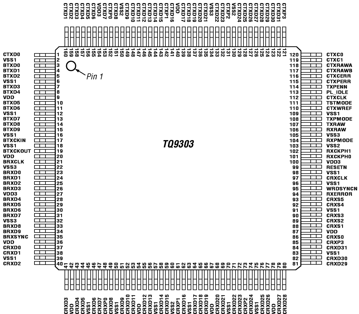
Figure 6. Pinout
