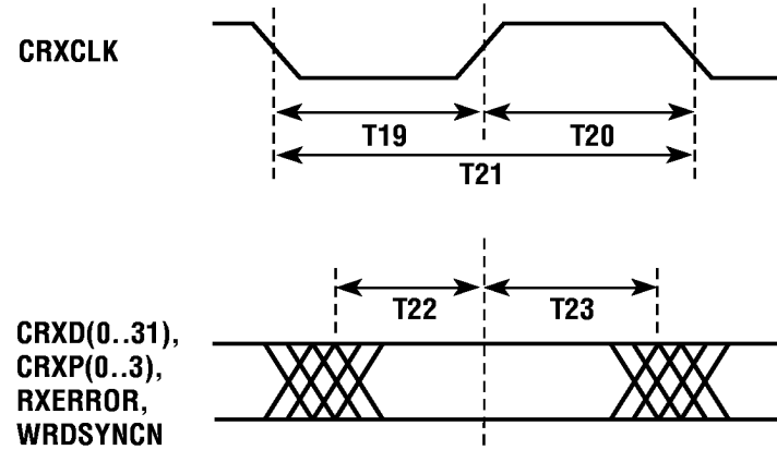
Figure 10. Receive (CRX) Timing
