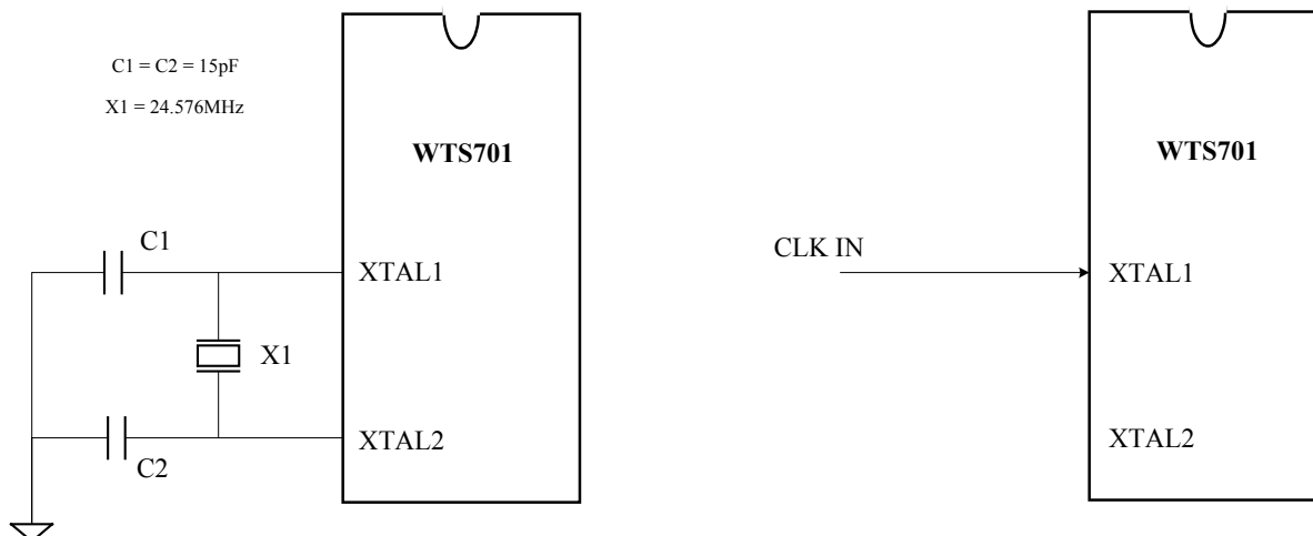
Figure 6. Clock Generation.
