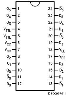
28-Pin PCC
