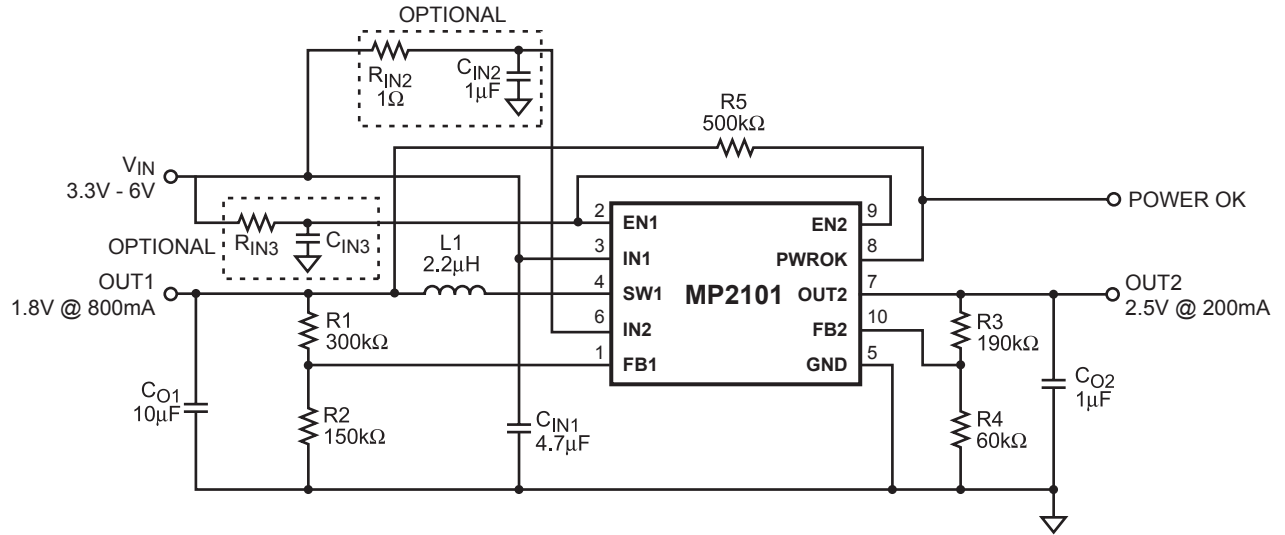
Figure 2—Optional RC Delay on EN1 and EN2 Circuit
