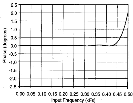
Figure 24. DAC Phase Response.
