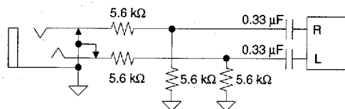
Figure 2. Line Inputs
