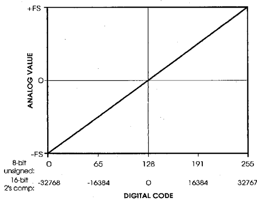
Figure 14. Linear Transfer Functions
