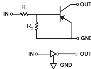
SCHMATIC DIAGRAM
