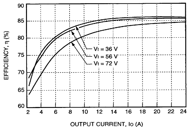
Figure 4. Typical FW150S6R5 Efficiency vs. Output Current at Room Temperature
