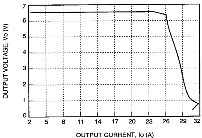
Figure 2. Typical FW150S6R5 Output Characteristics at Room Temperature and 48 V Input
