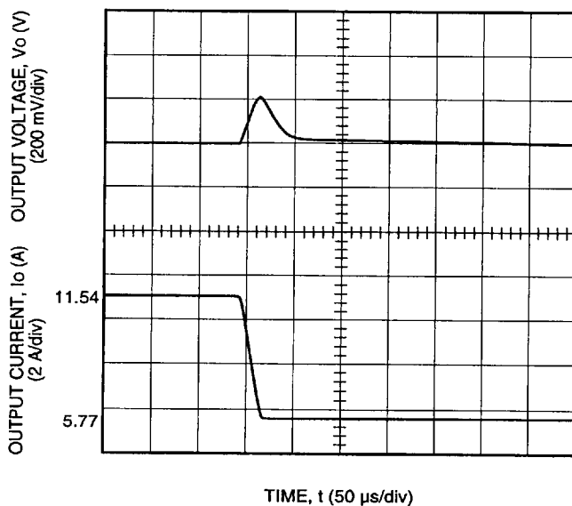
Figure 6. Typical FW150S6R5 Transient Response to Step Decrease in Load from 50% to 25% of Full Load at Room Temperature and 48 V Input (Waveform Averaged to Eliminate Ripple Component.)
