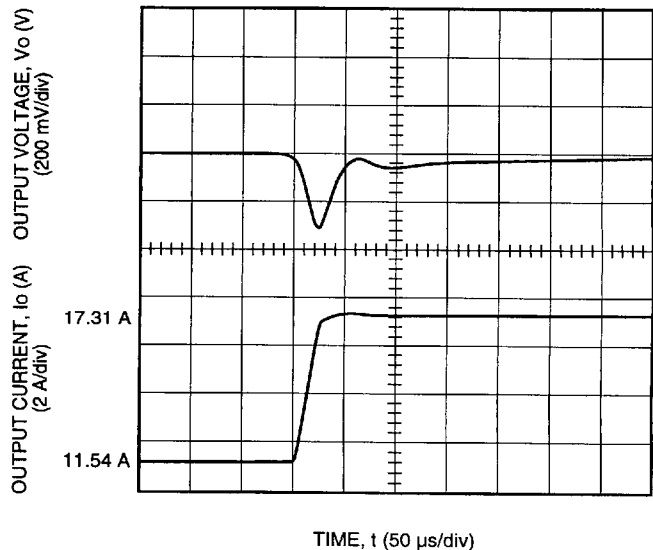
Figure 7. Typical FW150S6R5 Transient Response to Step Increase in Load from 50% to 75% of Full Load at Room Temperature and 48 V Input (Waveform Averaged to Eliminate Ripple Component.)
