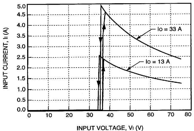
Figure 1. Typical FW150S6R5 Input Characteristics at Room Temperature
