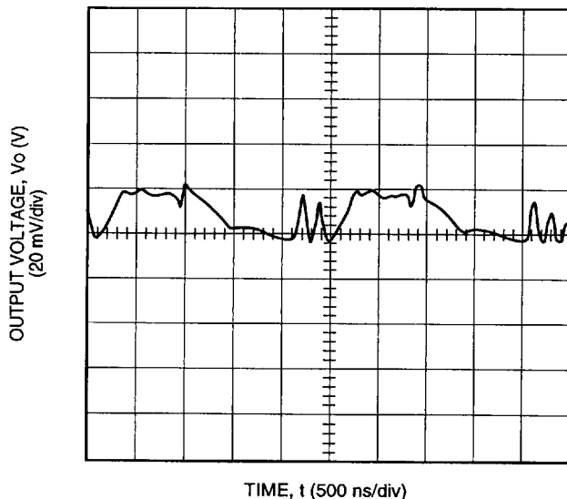
Figure 5. Typical FW150S6R5 Output Ripple Voltage at Room Temperature, 48 V Input, and 23.1 A Output
