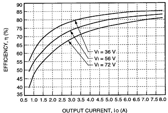
Figure 3. Typical FW050S6R5 Efficiency vs. Output Current at Room Temperature
