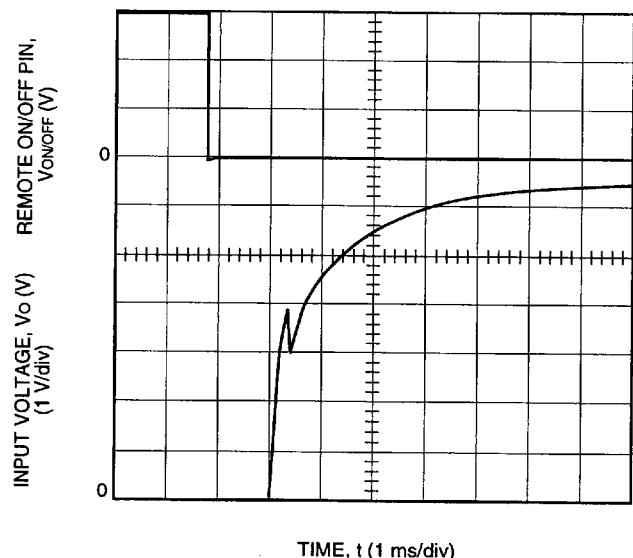
Figure 8. Typical FW050S6R5 Start-Up Transient at Room Temperature, 48 V Input, and 23.1 A Output
