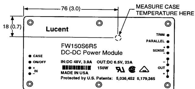
Figure 18. Case Temperature Measurement Location
