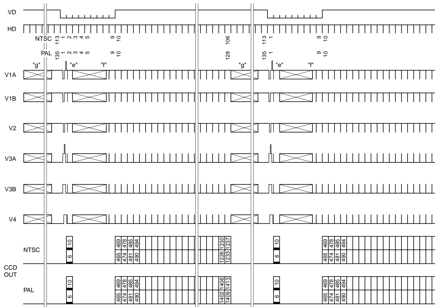
Drive Timing Chart (Vertical Sync) NTSC/PAL AF1 Mode NTSC: 60 frame/s, PAL: 50 frame/s
