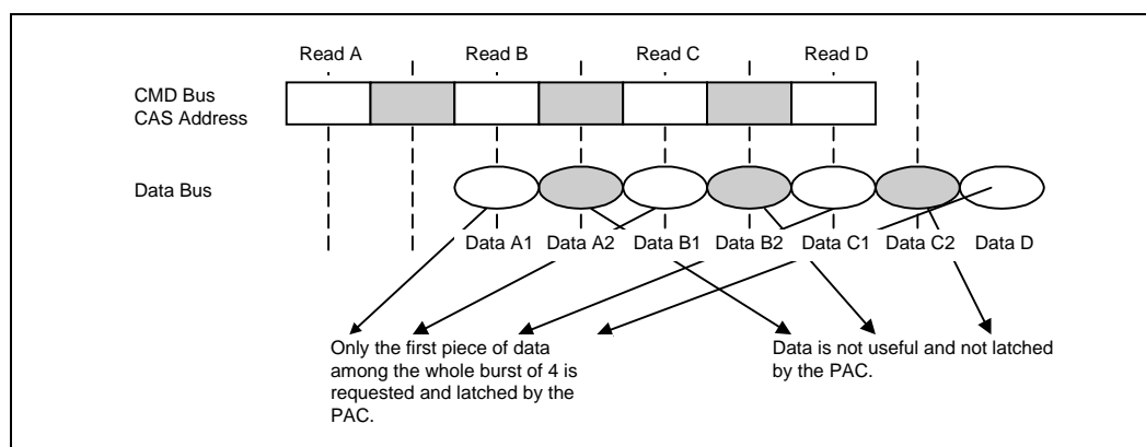
Figure 4-3. Single Clock Mode Disabled
