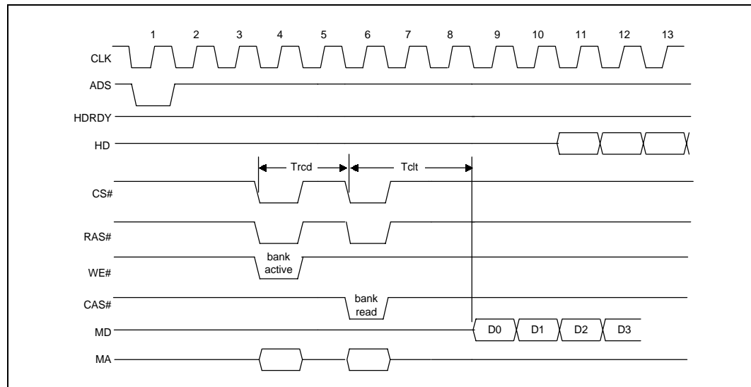
Figure 5-14. Row Miss-4 with SCLT=0, SRCD=1, SRPT=1
