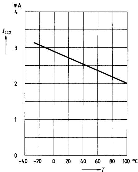
I_{CC2} Standby current vs. temperature (typ.)
