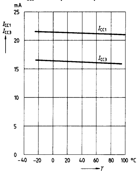
I_{CC} (Average) vs. Temperature (typ.)
