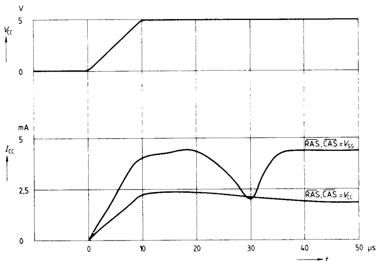
Current Consumption During Power up ( V_{\text{CC}} rise time 10 \mu\text{s} )
