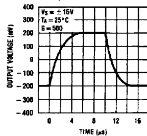
Small Signal Transient Response
