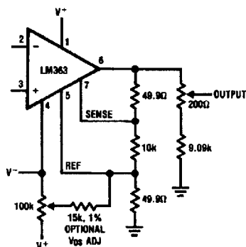
FIGURE 5. Adjusting Gain, Alternate Technique
