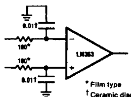
FIGURE 2. Low Pass Filter Prevents RF Rectification
