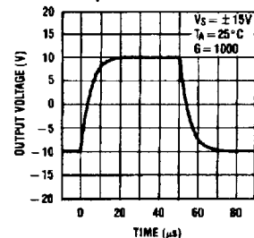
Large Signal Transient Response
