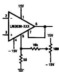
b. Output Offset Adj. for 8-Pin Package
