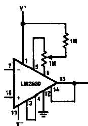
a. Input Offset Adj. for 16-Pin Package
