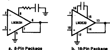
FIGURE 6. Overcompensation
