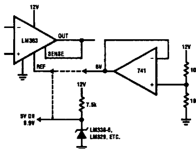
d. Single Supply, Bipolar Output
