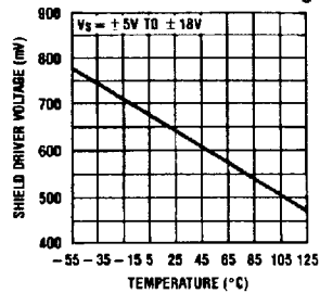
Shield Driver Bias Voltage
