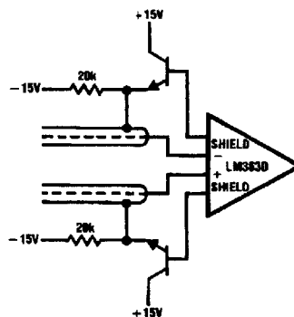
b. NPN Followers to Reduce Offsets
