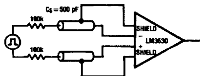
FIGURE 9. Improved Response using Shield Drivers
