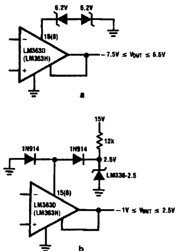
FIGURE 7. Output Clamp
