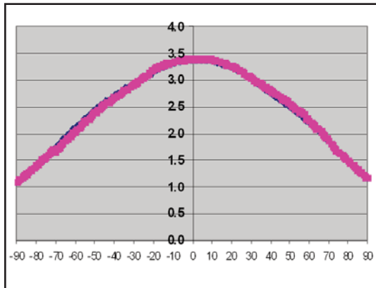
Intensity (cd) vs. Viewing Angle TB2-8111-001 (Blue)
