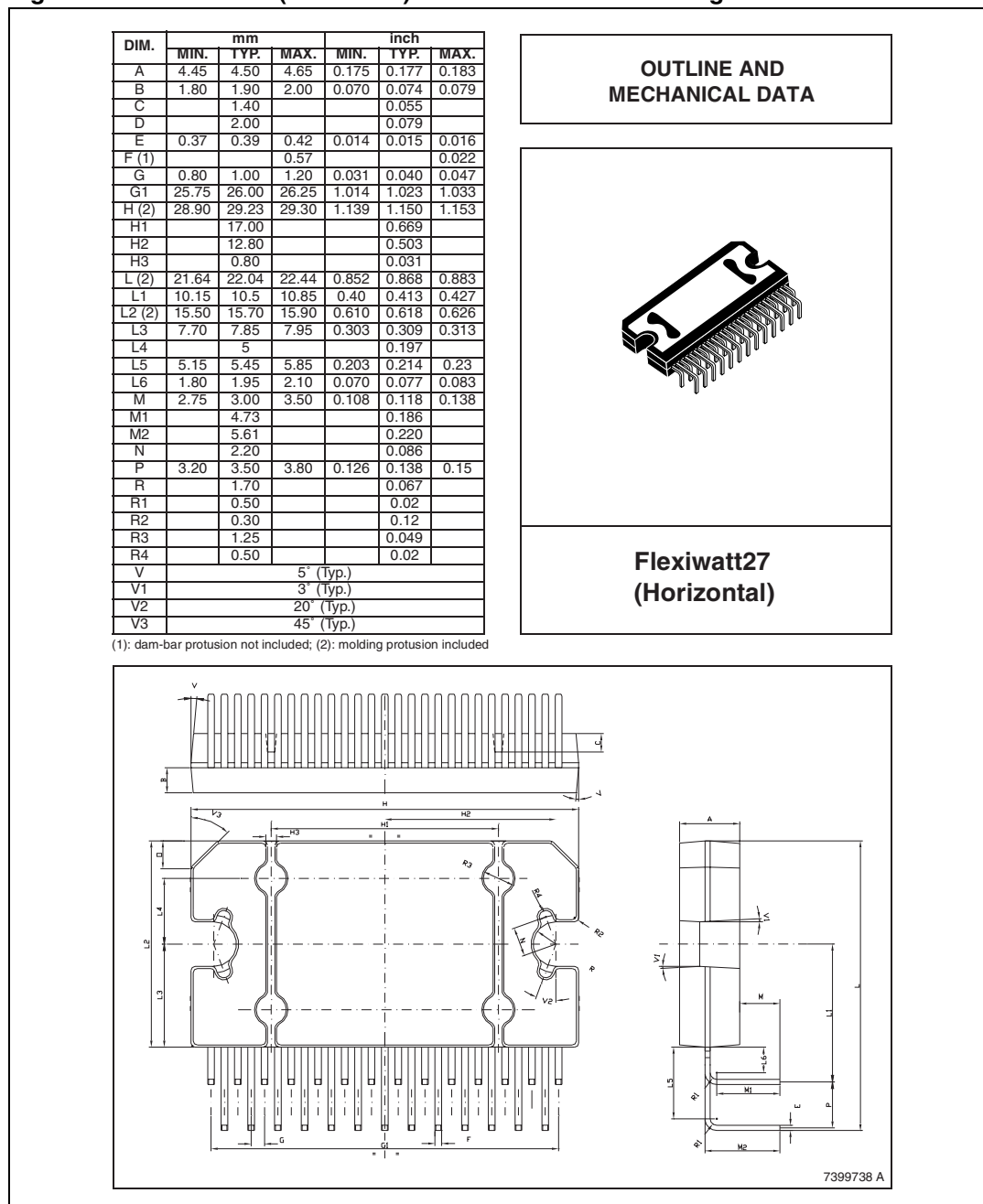
Figure 32. Flexiwatt27 (horizontal) Mechanical Data & Package Dimensions
