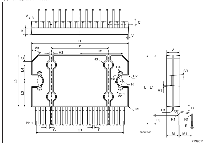
Flexiwatt27 (vertical)
