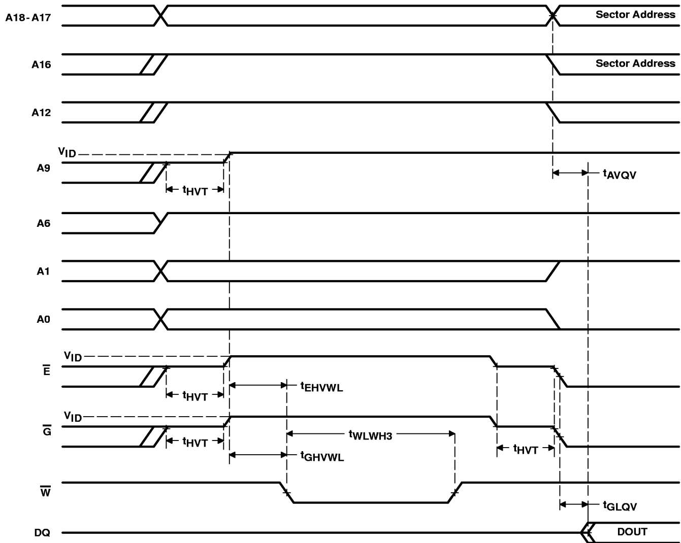
Figure 17. AC Waveform for Sector-Unprotect Operation
