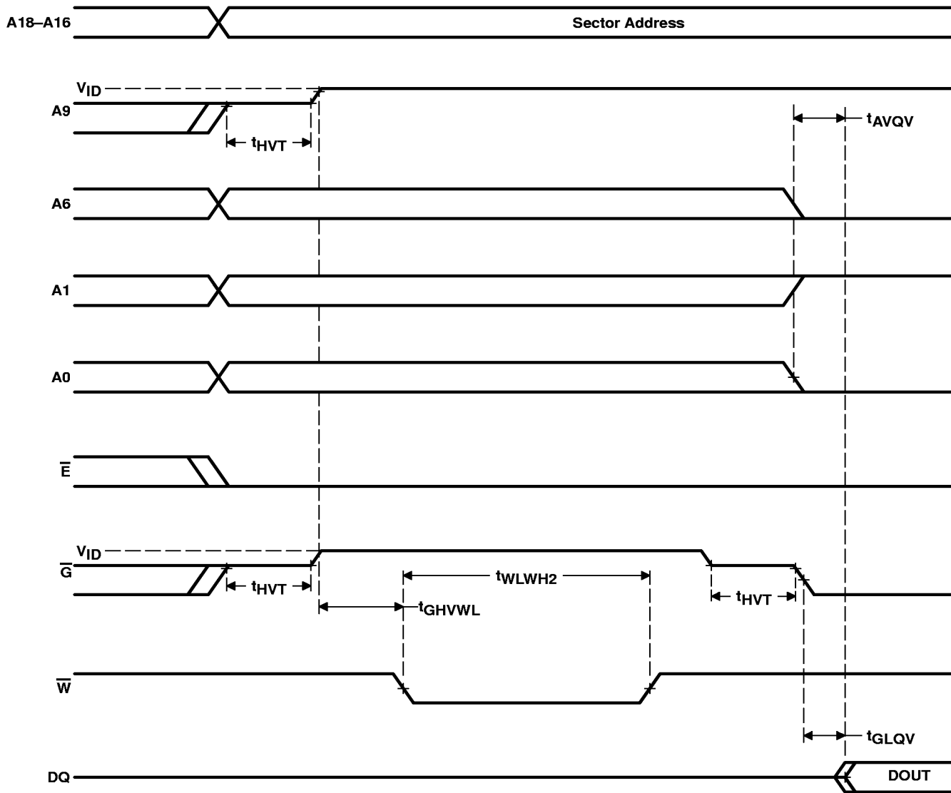
Figure 15. AC Waveform for Sector-Protect Operation
