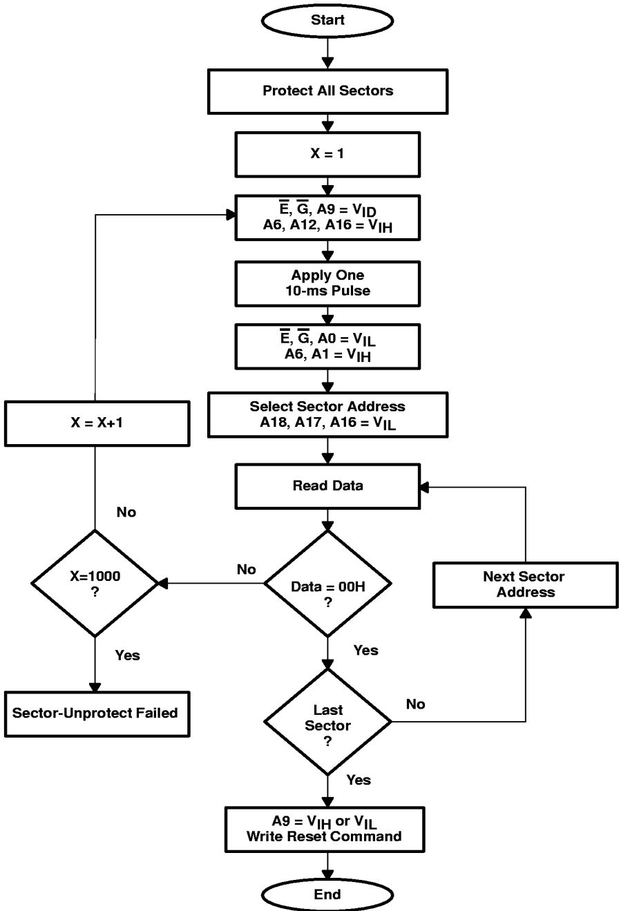
Figure 16. Sector-Unprotect Algorithm
