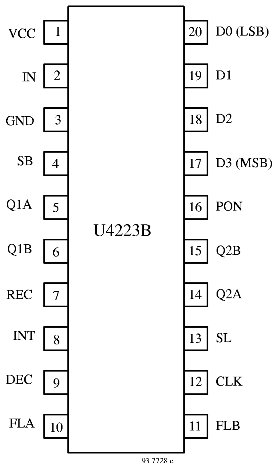
Figure 2. Pinning
