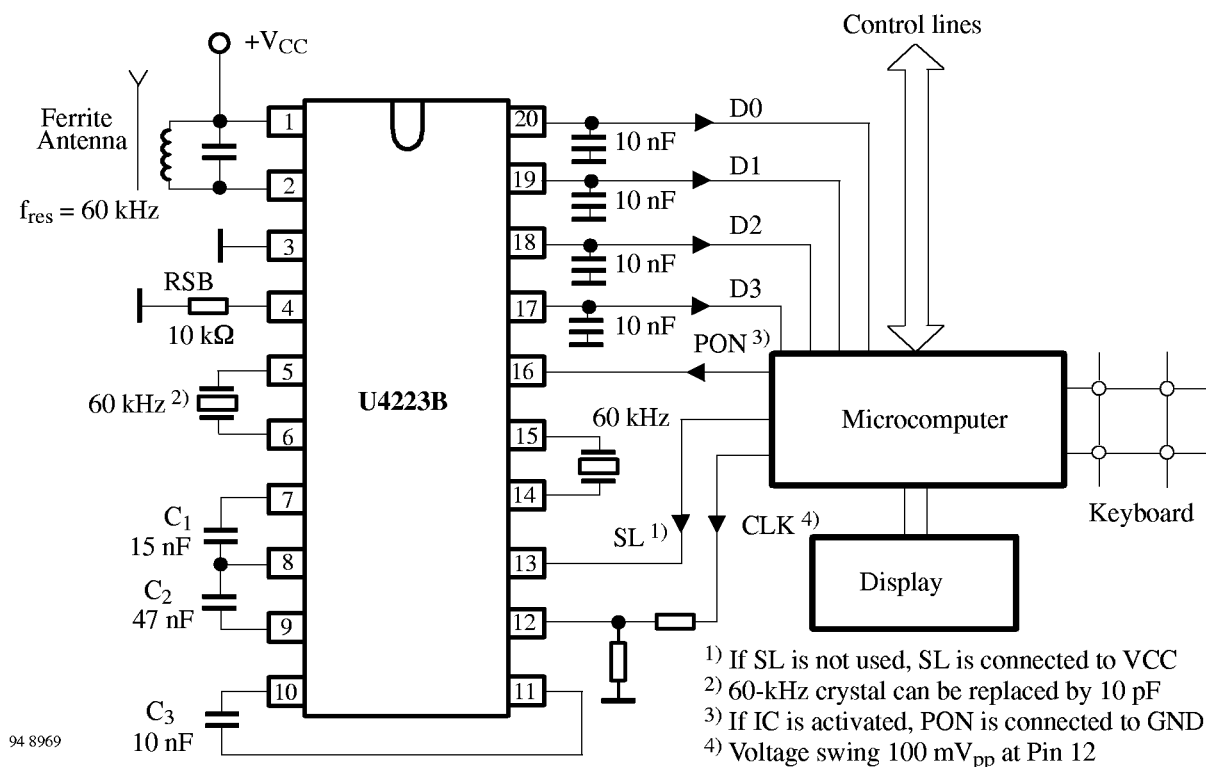
Application Circuit for WWVB 60 kHz
