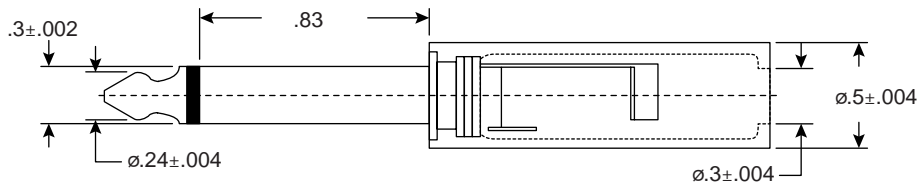
DIMENSIONS (IN.)
