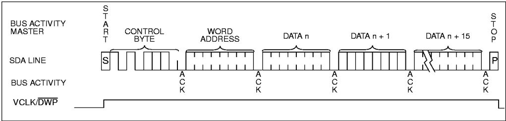
FIGURE 4-2: PAGE WRITE
