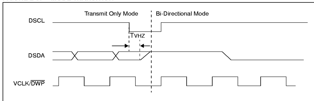
FIGURE 2-3: MODE TRANSITION
