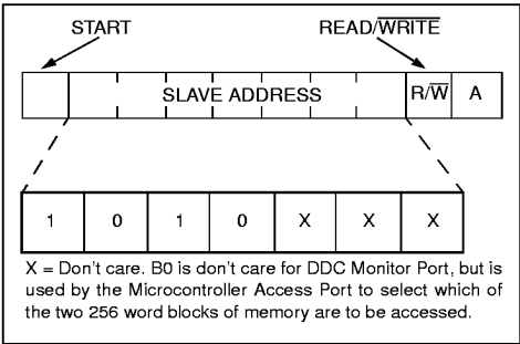
FIGURE 3-4: CONTROL BYTE ALLOCATION
