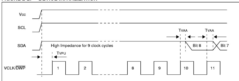
FIGURE 2-2: DEVICE INITIALIZATION
