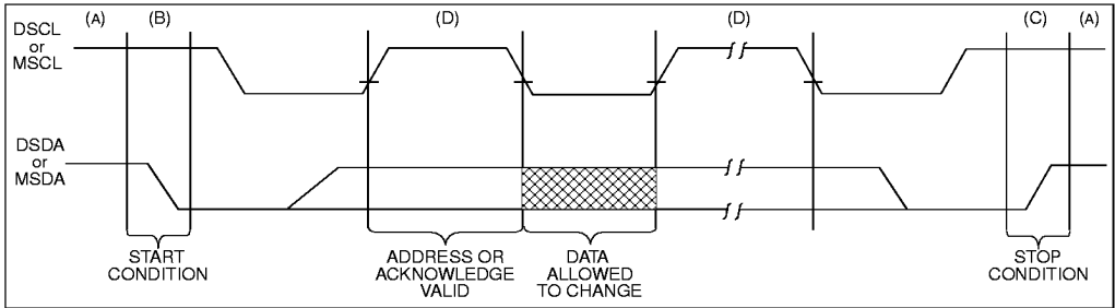
FIGURE 3-2: BUS TIMING START/STOP
